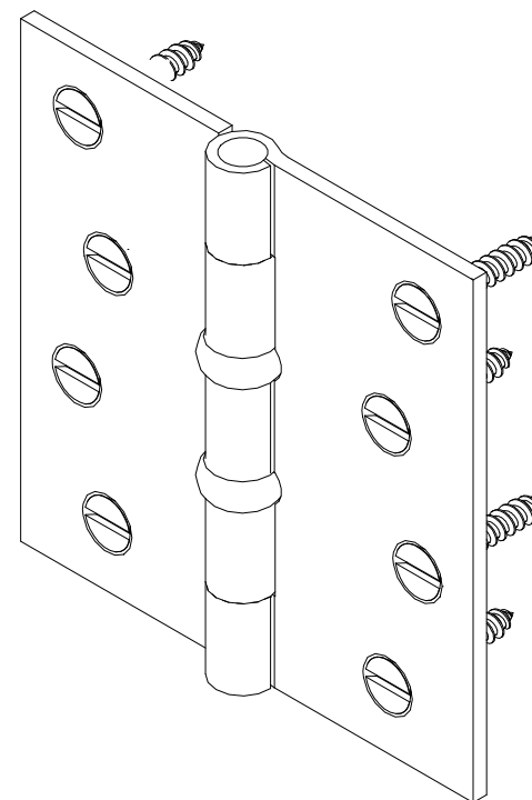
3 ISOMETRIC VIEW
