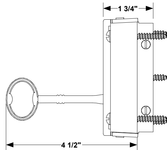
2 SIDE VIEW
