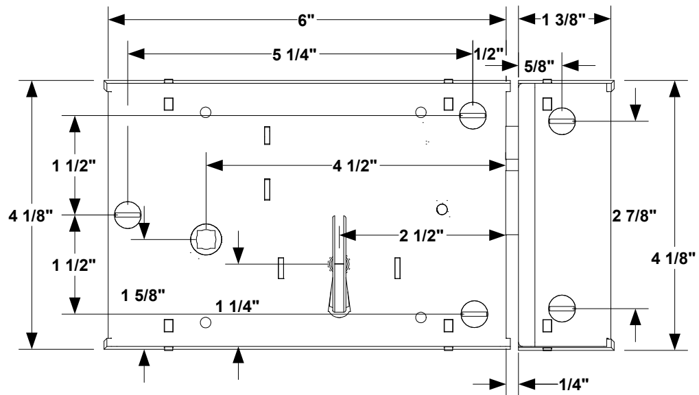
1 FRONT VIEW
