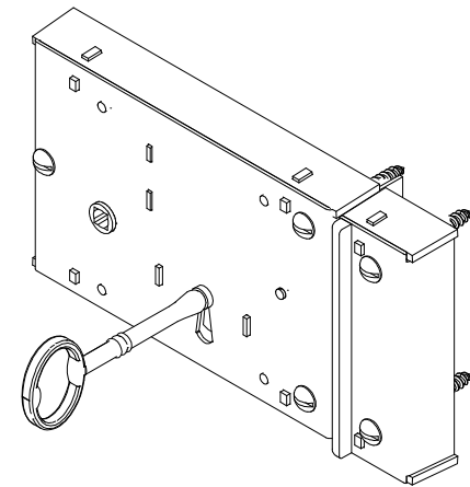
3 ISOMETRIC VIEW
