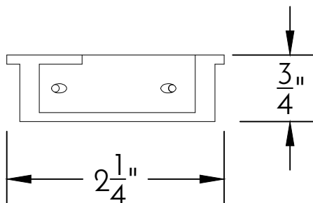
1 FRONT VIEW
