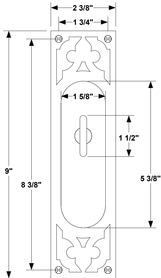
1 FRONT VIEW
