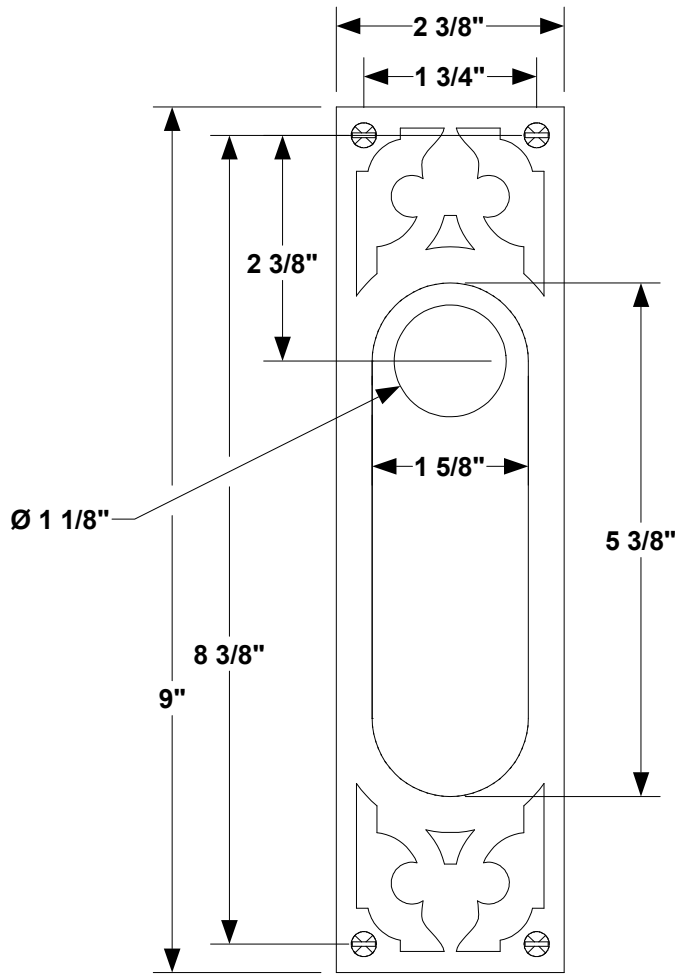
1 FRONT VIEW
