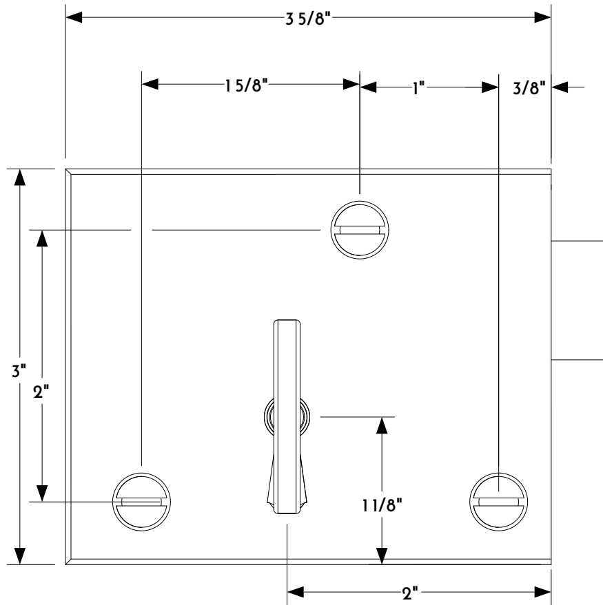
1 FRONT VIEW
