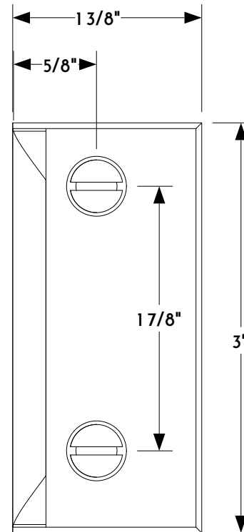
2 TOP VIEW
