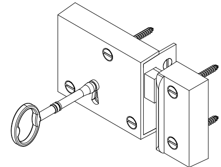
3 ISOMETRIC VIEW
