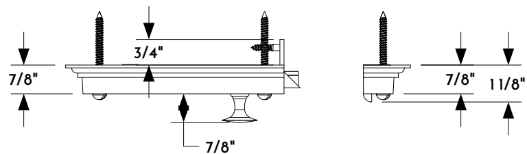
1 TOP VIEW
