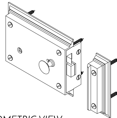
3 ISOMETRIC VIEW
