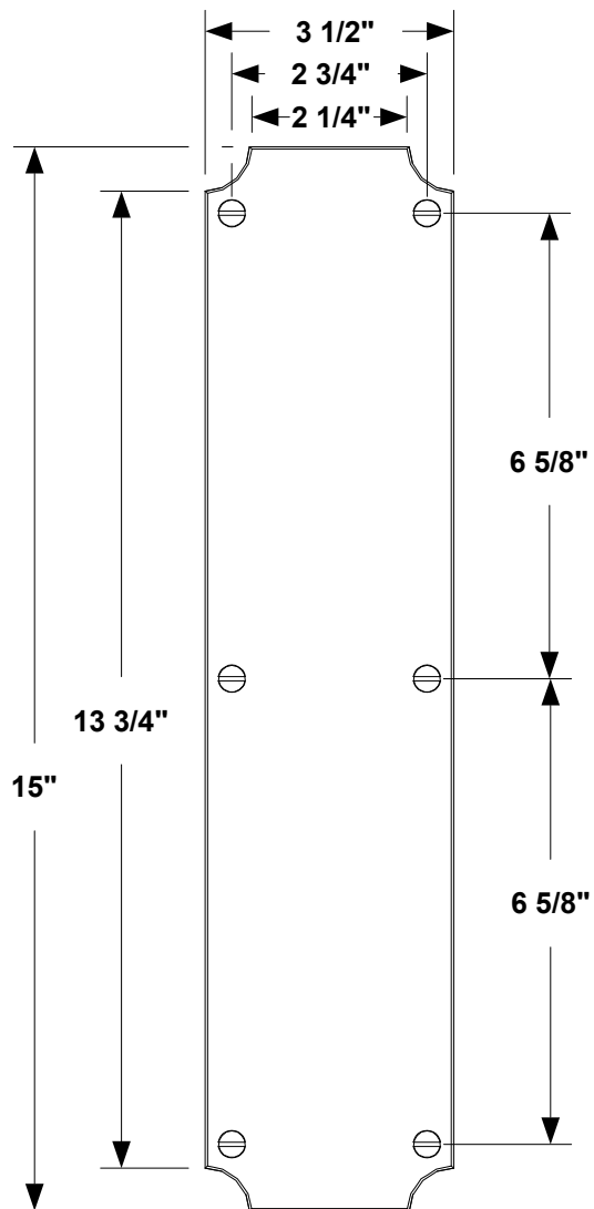
1 FRONT VIEW
