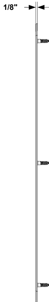
2 SIDE VIEW
