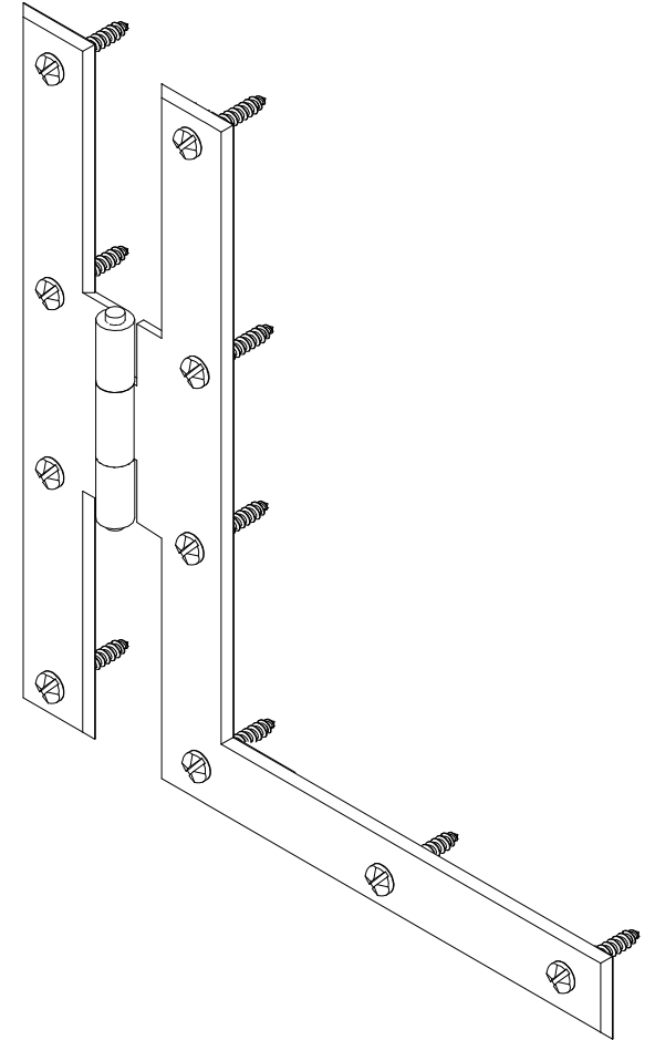
3 ISOMETRIC VIEW
