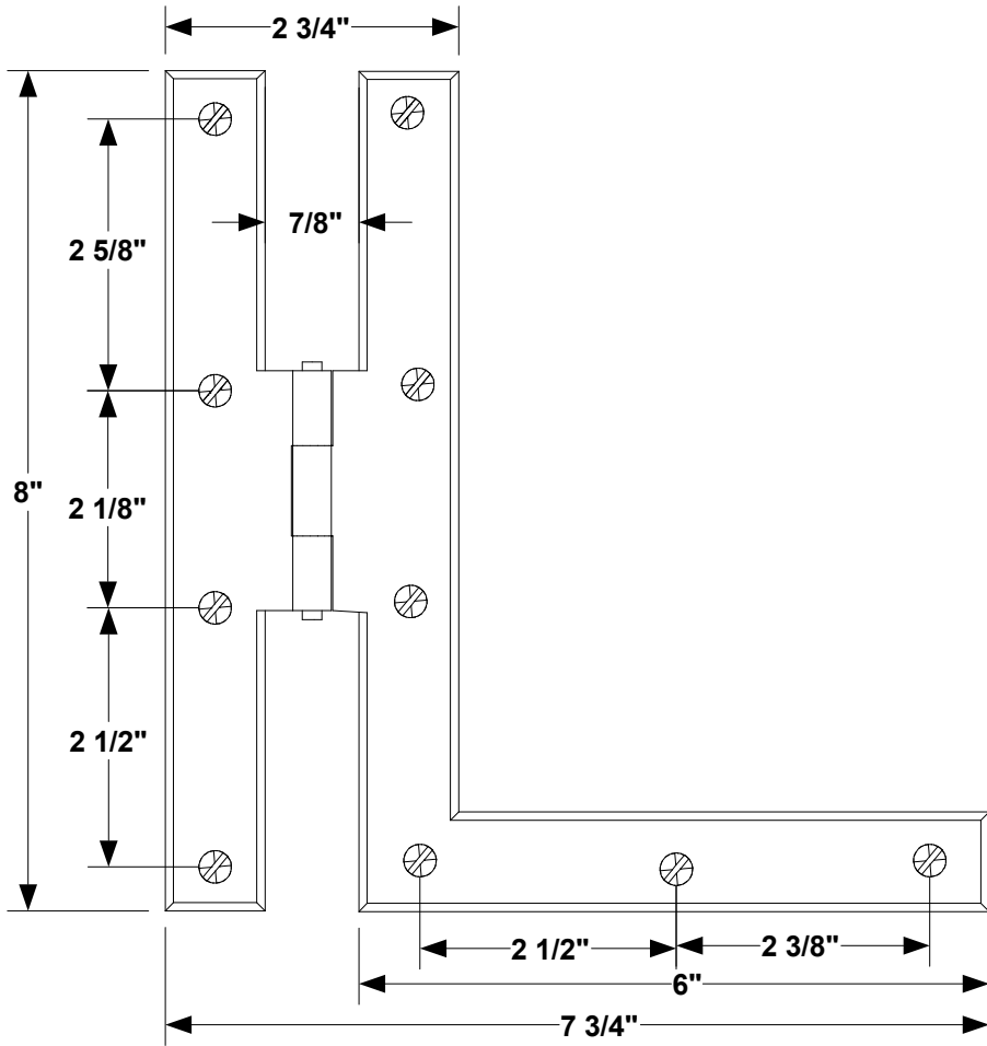
1 FRONT VIEW
