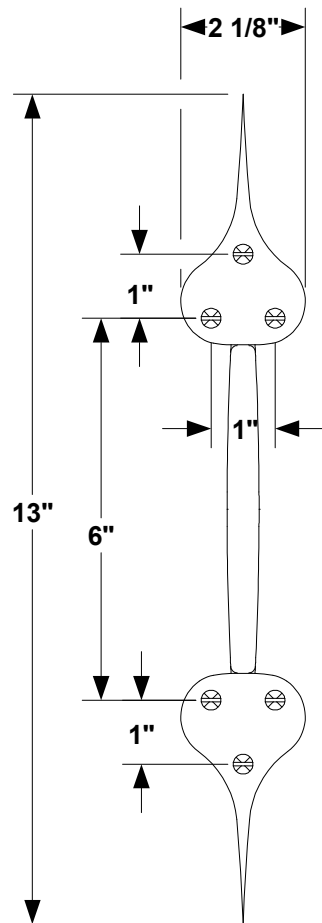
1 FRONT VIEW
