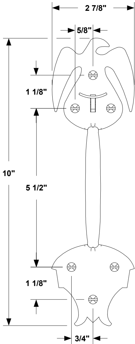
1 FRONT VIEW
