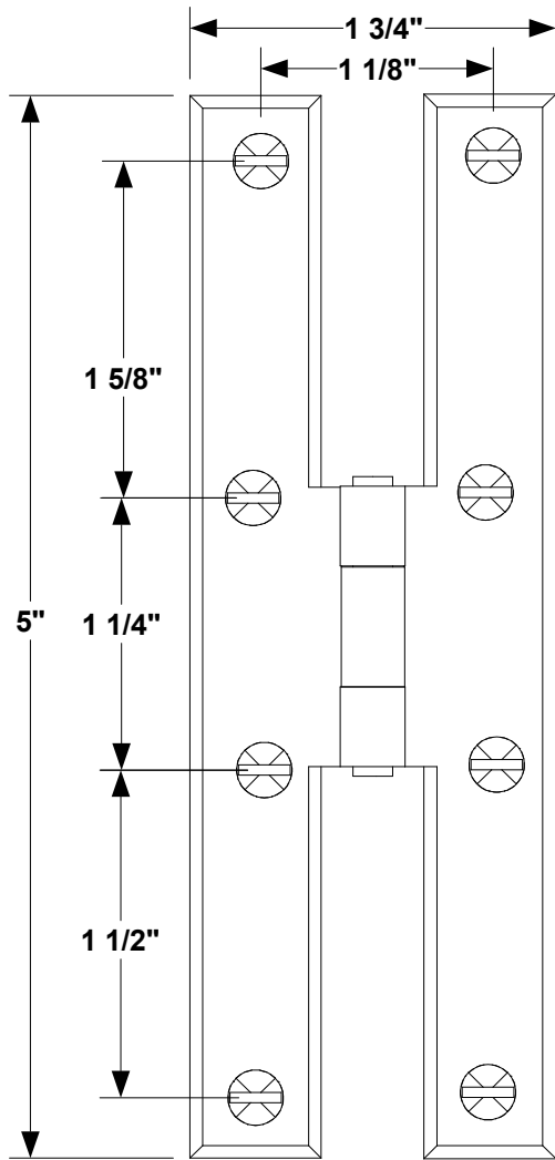
① FRONT VIEW
