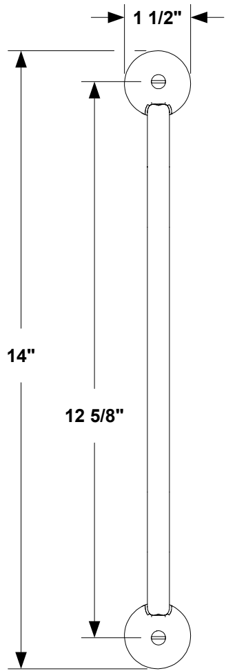
1 FRONT VIEW
