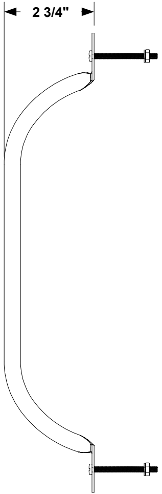
2 SIDE VIEW
