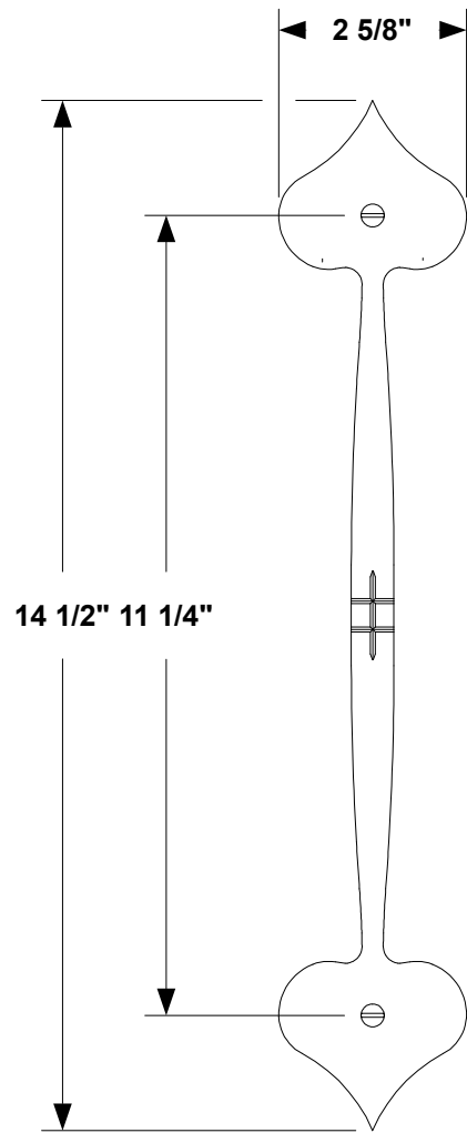
1 FRONT VIEW
