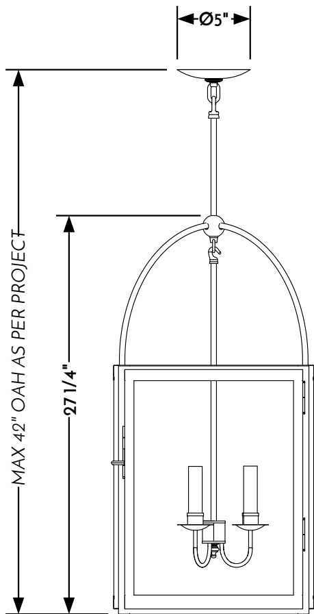
① HANGING LANTERN FRONT ELEVATION VIEW
