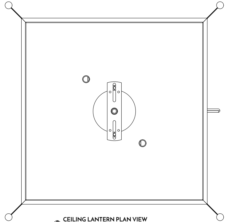
② CEILING LANTERN PLAN VIEW
