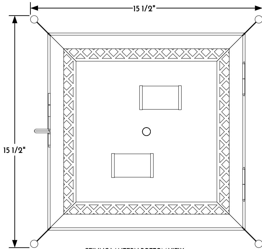
① CEILING LANTERN BOTTOM VIEW
