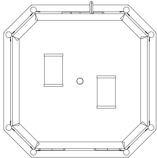
② CEILING LANTERN BOTTOM VIEW
