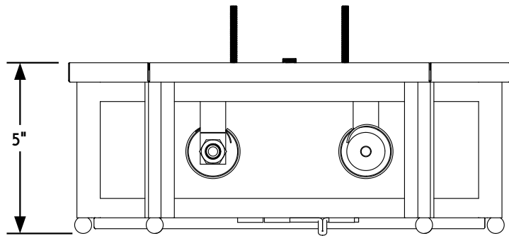
③ CEILING LANTERN ELEVATION VIEW
