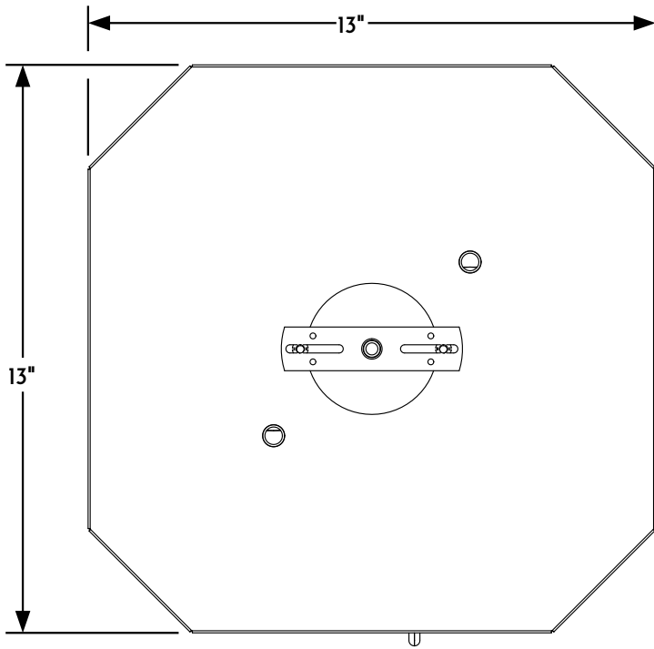
① CEILING LANTERN PLAN VIEW
