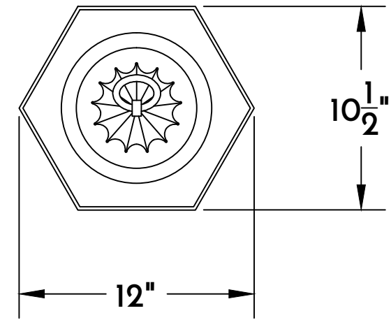
② LANTERN TOP PLAN VIEW
