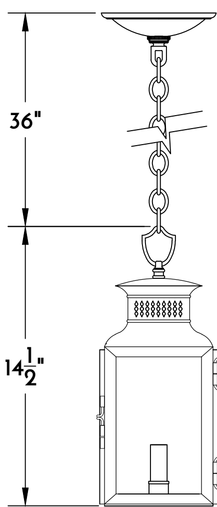
① HANGING LANTERN SIDE ELE.
