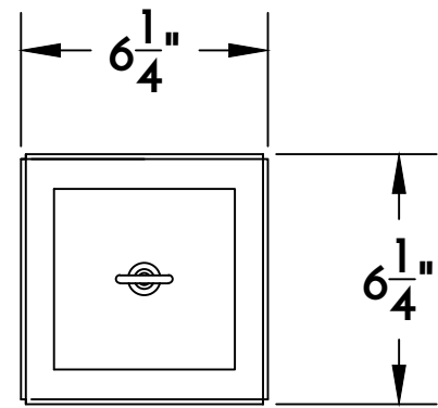
④ HANGING LANTERN TOP PLAN VIEW
