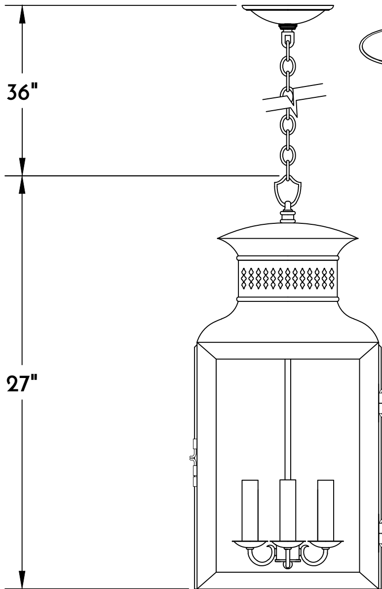
① HANGING LANTERN SIDE ELE.
