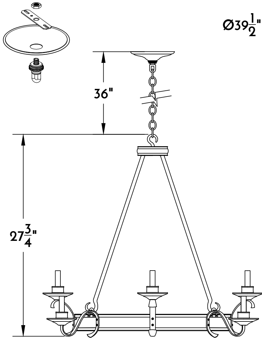
① CHANDELIER SIDE ELE.
