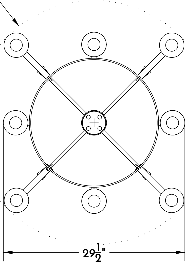
② CHANDELIER TOP PLAN VIEW
