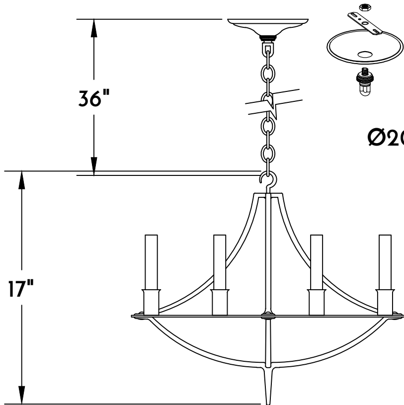
① CHANDELIER SIDE ELE.
