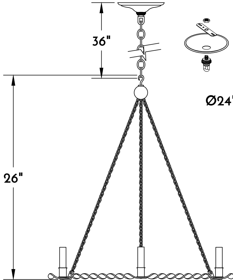
① CHANDELIER FRONT ELE.
