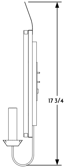
② WALL LANTERN RIGHT ELEVATION VIEW
