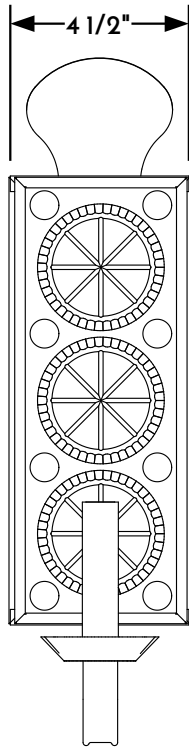
① WALL LANTERN FRONT ELEVATION VIEW
