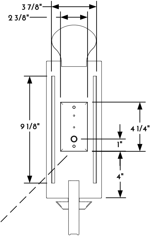
③ WALL LANTERN REAR ELEVATION VIEW
