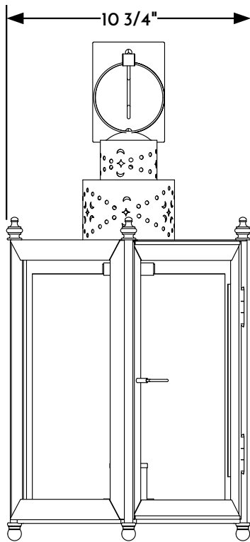
① WALL LANTERN FRONT ELEVATION VIEW
