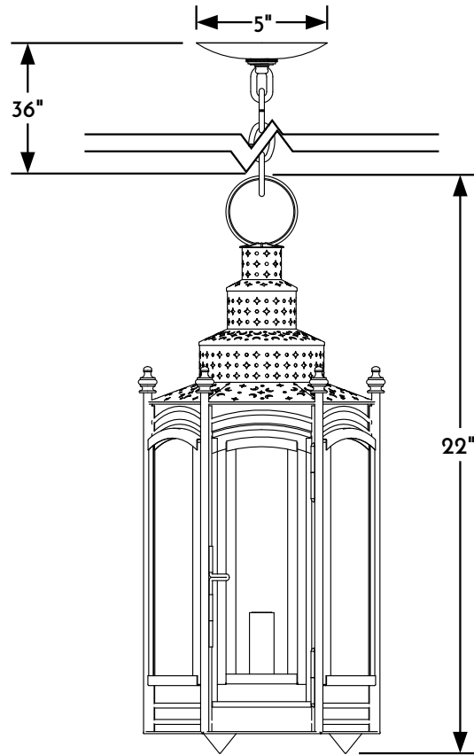
① HANGING LANTERN FRONT ELEVATION VIEW
