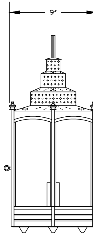
② HANGING LANTERN RIGHT ELEVATION VIEW
