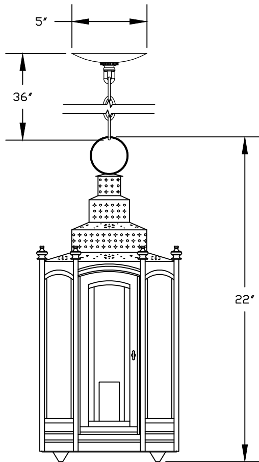
① HANGING LANTERN FRONT ELEVATION VIEW
