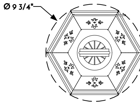
③ HANGING LANTERN PLAN VIEW
