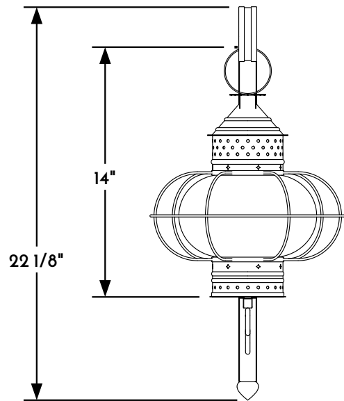
① WALL LANTERN FRONT ELEVATION VIEW
