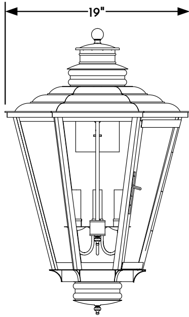
① WALL LANTERN FRONT ELEVATION VIEW
