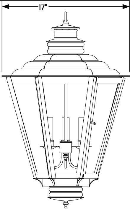
① HANGING LANTERN FRONT ELEVATION VIEW
