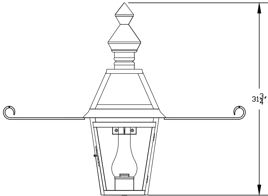
① WALL LANTERN FRONT ELEVATION VIEW
