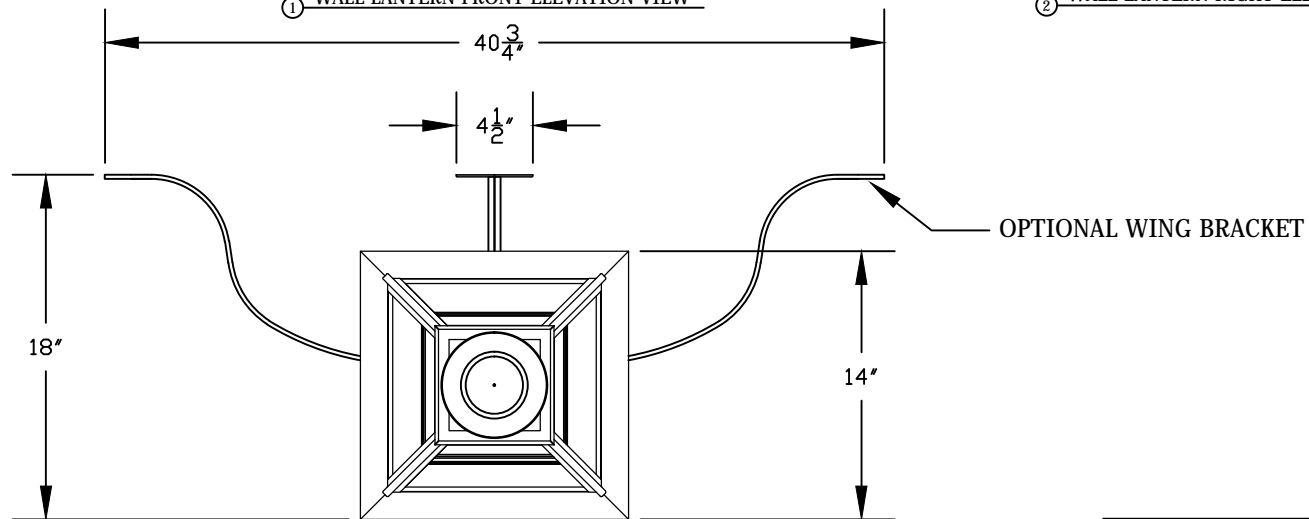
③ WALL LANTERN PLAN VIEW
