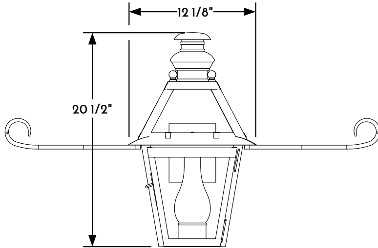
① WALL LANTERN FRONT ELEVATION VIEW
