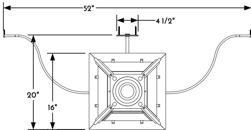
④ WALL LANTERN PLAN VIEW
