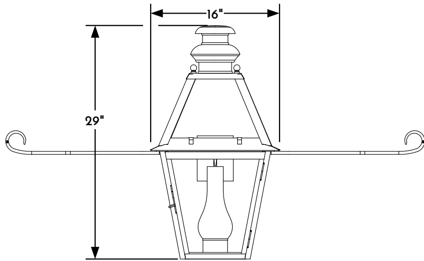
① WALL LANTERN FRONT ELEVATION VIEW
