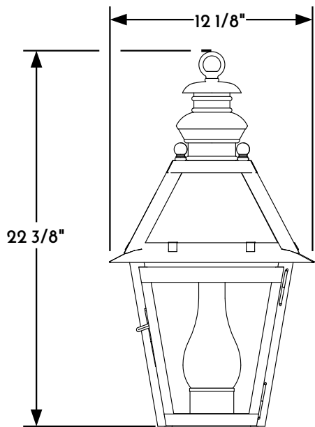
① HANGING LANTERN FRONT ELEVATION VIEW
