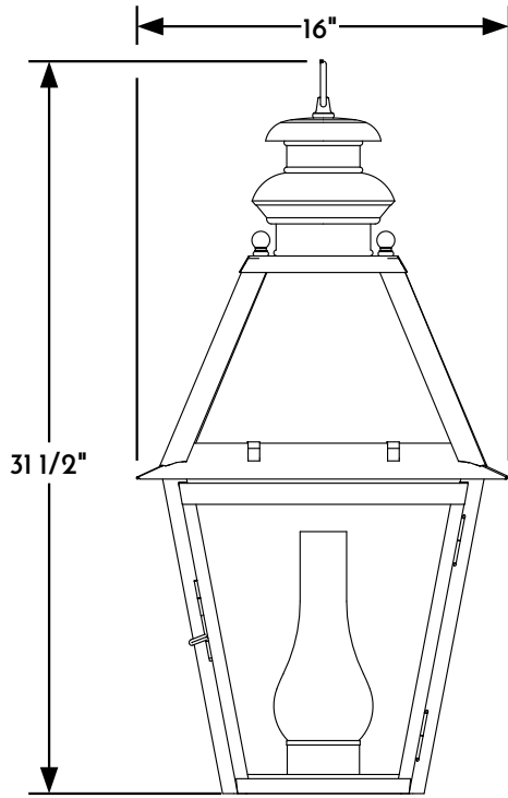
① HANGING LANTERN FRONT ELEVATION VIEW
