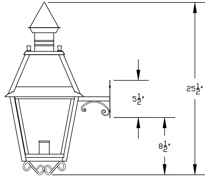
② WALL LANTERN RIGHT ELEVATION VIEW
