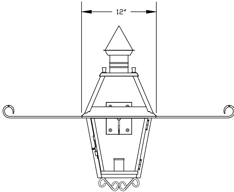
① WALL LANTERN FRONT ELEVATION VIEW
