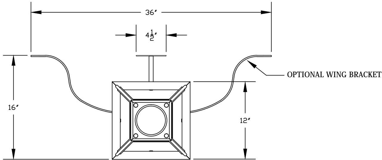
③ WALL LANTERN PLAN VIEW
