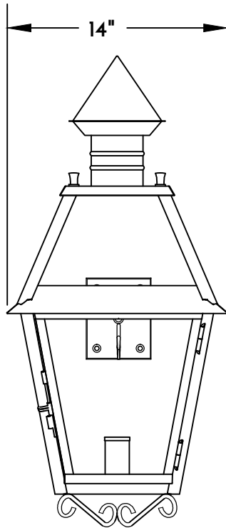
① WALL LANTERN FRONT ELEVATION VIEW
