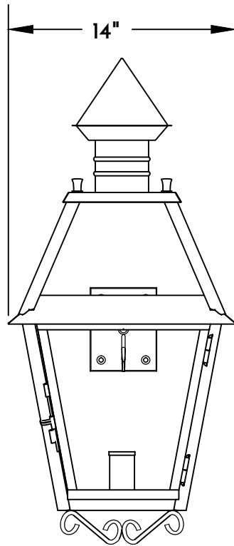
1 WALL LANTERN FRONT ELEVATION VIEW
