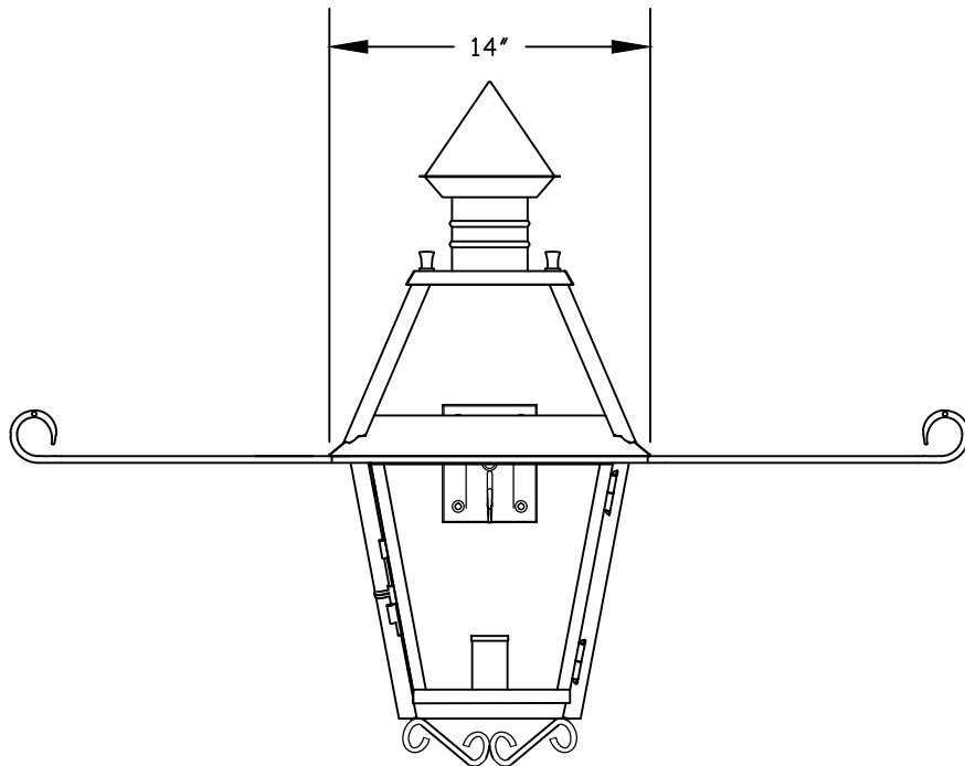
1 WALL LANTERN FRONT ELEVATION VIEW
