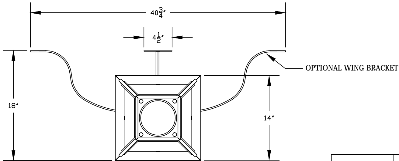
3 WALL LANTERN PLAN VIEW
