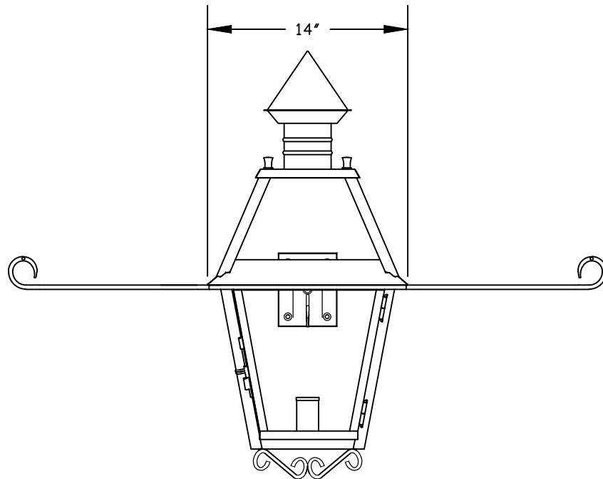
1 WALL LANTERN FRONT ELEVATION VIEW
