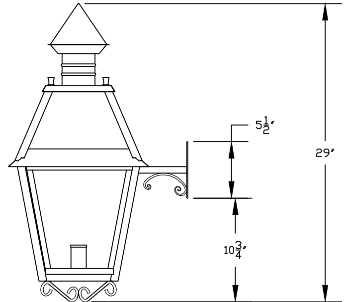
2 WALL LANTERN RIGHT ELEVATION VIEW
