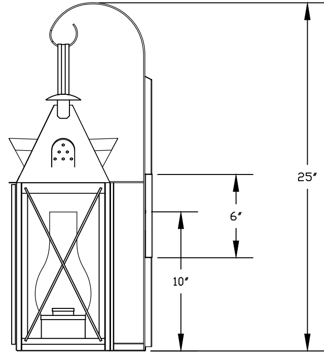
② WALL LANTERN RIGHT ELEVATION VIEW
