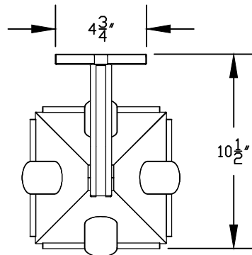
① WALL LANTERN FRONT ELEVATION VIEW
