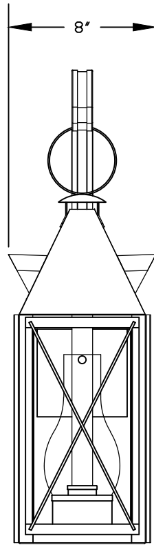
① WALL LANTERN FRONT ELEVATION VIEW
