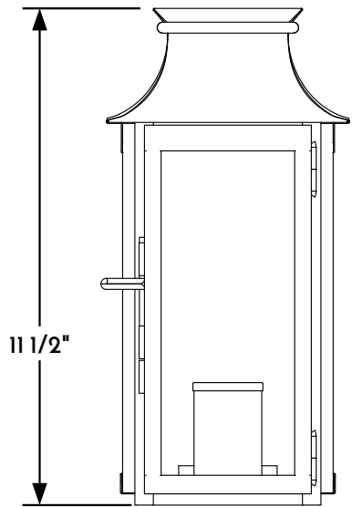
① WALL LANTERN FRONT ELEVATION VIEW
