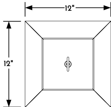
④ HANGING LANTERN PLAN VIEW
