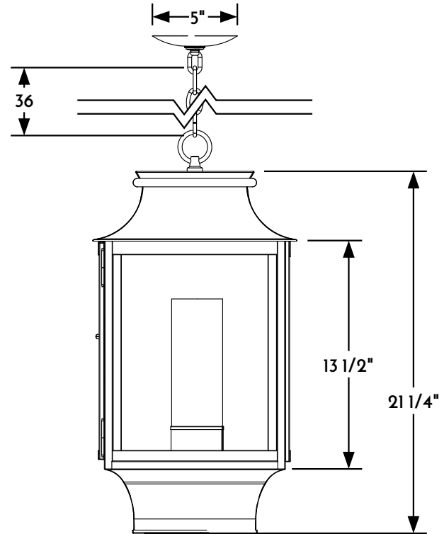
② HANGING LANTERN RIGHT VIEW
