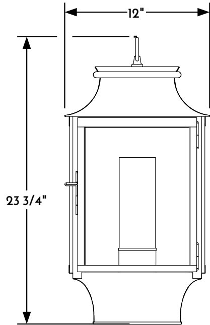
① HANGING LANTERN ELEVATION VIEW
