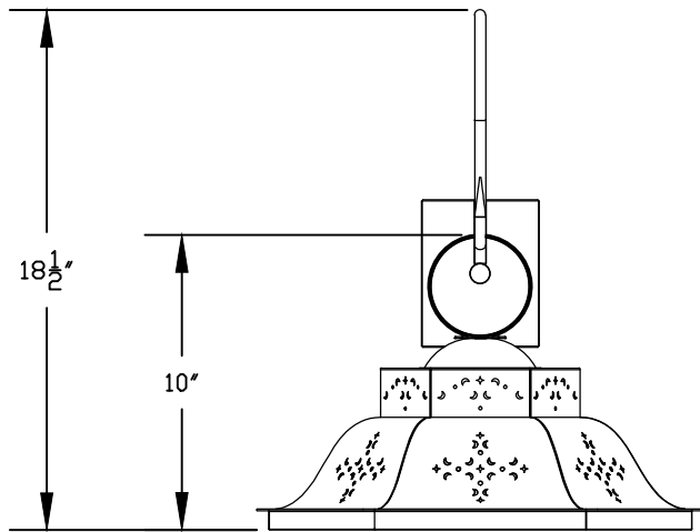
1 WALL PENDANT FRONT ELEVATION VIEW
