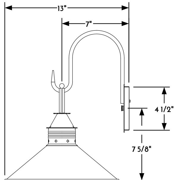
② WALL PENDANT RIGHT ELEVATION VIEW
