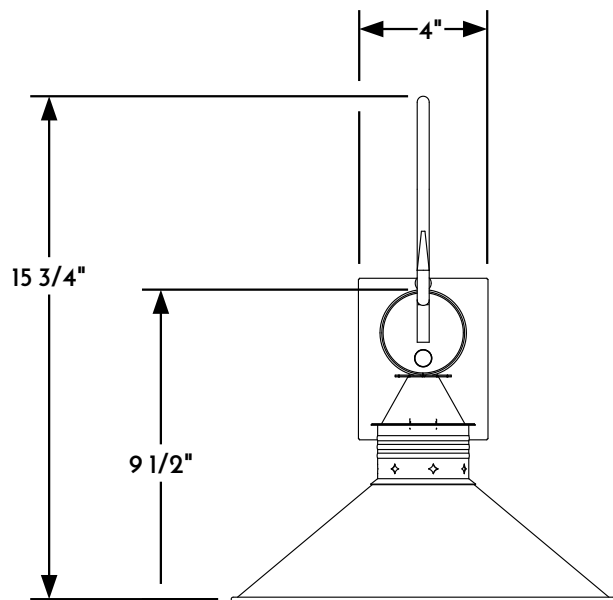
① WALL PENDANT FRONT ELEVATION VIEW
