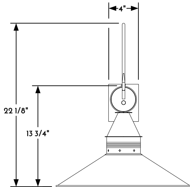
① WALL PENDANT FRONT ELEVATION VIEW
