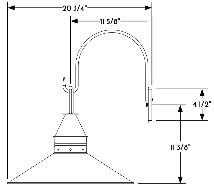
② WALL PENDANT RIGHT ELEVATION VIEW
