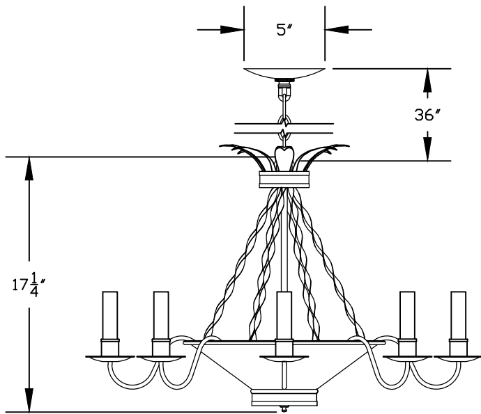
1 HANGING CHANDELIER ELEVATION VIEW
