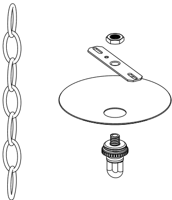
③ HANGING CHANDELIER CANOPY ASSEMBLY
