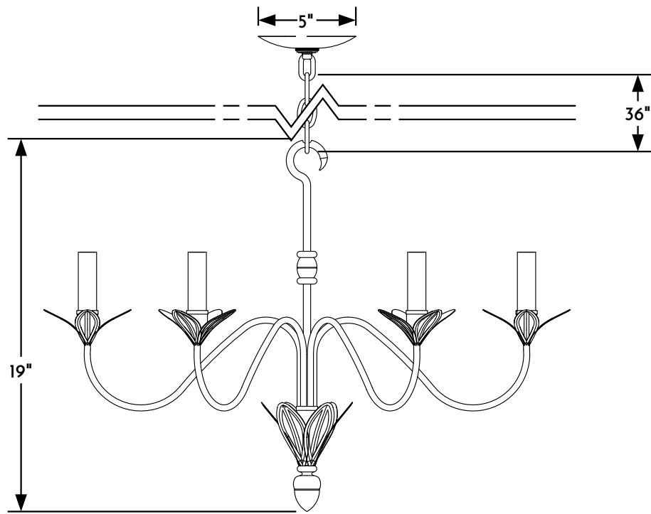
① HANGING CHANDELIER ELEVATION VIEW
