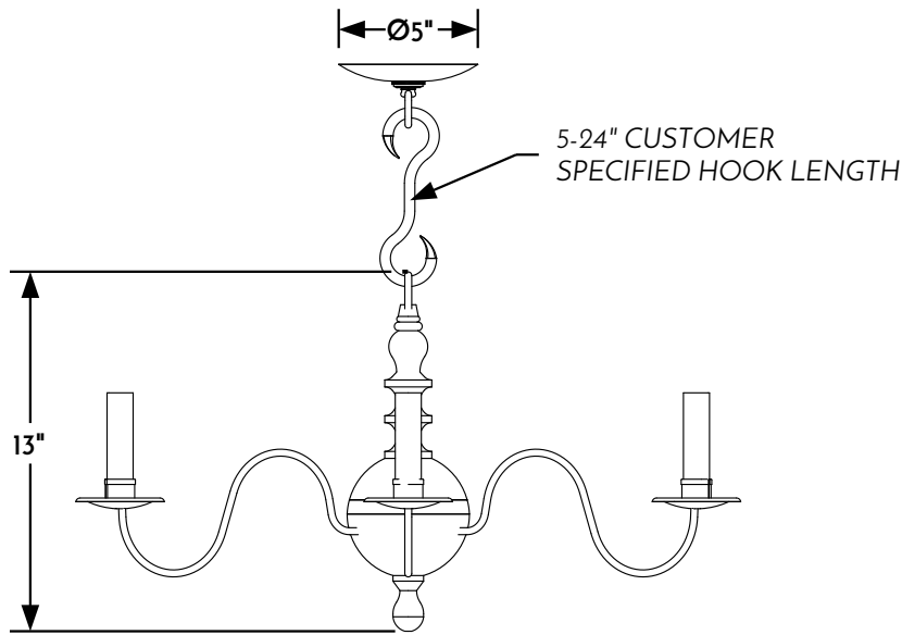
① HANGING CHANDELIER ELEVATION VIEW
