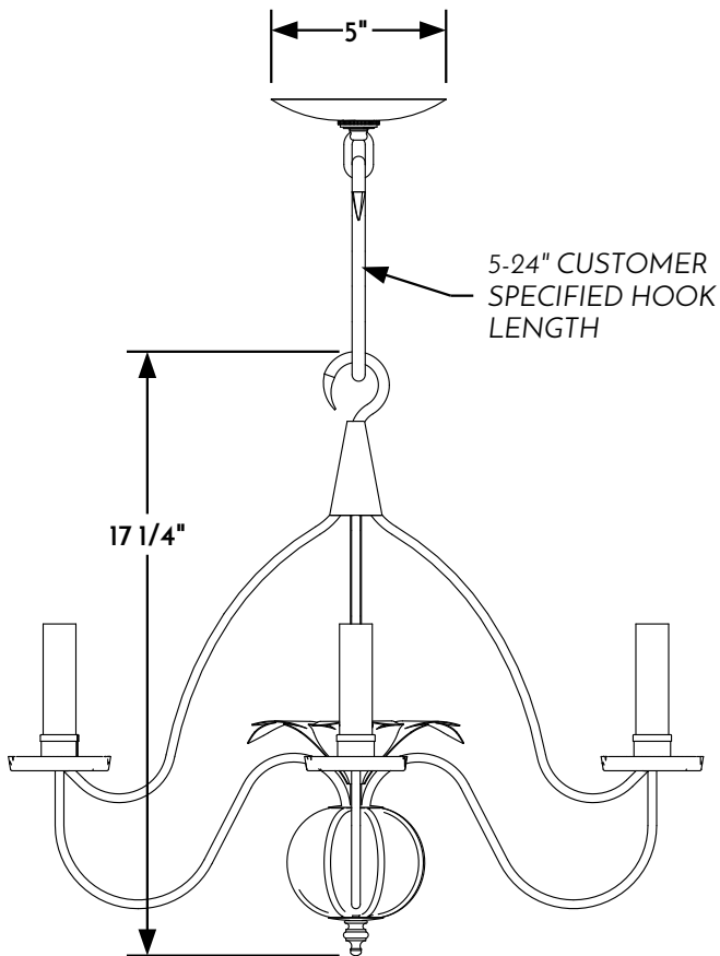
① HANGING CHANDELIER ELEVATION VIEW
