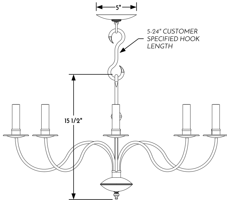
① HANGING CHANDELIER ELEVATION VIEW
